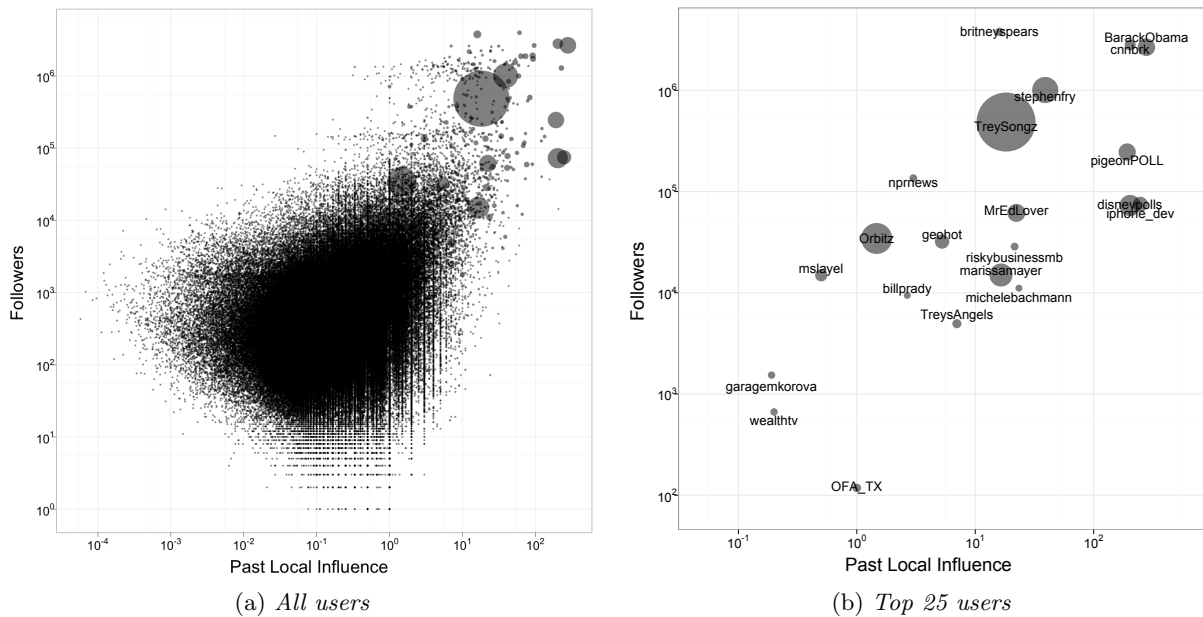
Figure 6: Influence as a function of past local influence and number of followers for (a) all users and (b) users with the top 25 actual influence. Each circle represents a single seed user, where the size of the circle represents that user’s actual average influence.
